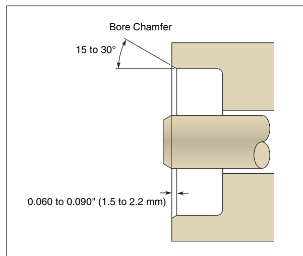
Figure 6-2. Housing Profile
